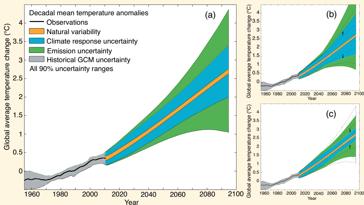
FAQ 1.1, Figure 1 | Schematic diagram showing the relative importance of different uncertainties, and their evolution in time. (a) Decadal mean surface temperature change (°C) from the historical record (black line), with climate model estimates of uncertainty for historical period (grey), along with future climate projections and uncertainty. Values are normalised by means from 1961 to 1980. Natural variability (orange) derives from model interannual variability, and is assumed constant with time. Emission uncertainty (green) is estimated as the model mean difference in projections from different scenarios. Climate response uncertainty (blue-solid) is based on climate model spread, along with added uncertainties from the carbon cycle, as well as rough estimates of additional uncertainty from poorly modelled processes. Based on Hawkins and Sutton (2011) and Huntingford et al. (2009). (b) Climate response uncertainty can appear to increase when a new process is discovered to be relevant, but such increases reflect a quantification of previously unmeasured uncertainty, or (c) can decrease with additional model improvements and observational constraints. The given uncertainty range of 90% means that the temperature is estimated to be in that range, with a probability of 90%.
