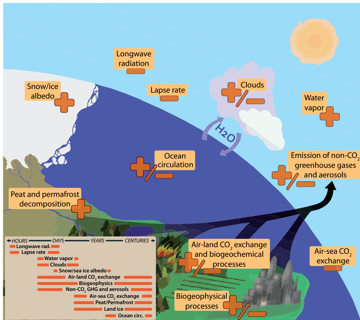
Figure 1.2 | Climate feedbacks and timescales. The climate feedbacks related to increasing \text{CO}_2 and rising temperature include negative feedbacks (–) such as LWR, lapse rate (see Glossary in Annex III), and air–sea carbon exchange and positive feedbacks (+) such as water vapour and snow/ice albedo feedbacks. Some feedbacks may be positive or negative (±): clouds, ocean circulation changes, air–land \text{CO}_2 exchange, and emissions of non-GHGs and aerosols from natural systems. In the smaller box, the large difference in timescales for the various feedbacks is highlighted.
