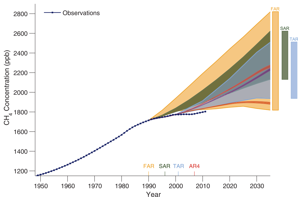
Figure 1.6 | Observed globally and annually averaged \text{CH}_4 concentrations in parts per billion (ppb) since 1950 compared with projections from the previous IPCC assessments. Estimated observed global annual \text{CH}_4 concentrations are shown in dark blue. The shading shows the largest model projected range of global annual \text{CH}_4 concentrations from 1950 to 2035 from FAR (Figure A.3 of the Annex of IPCC, 1990); SAR (Table 2.5a in Schimel et al., 1996); TAR (Appendix II of IPCC, 2001); and from the A2, A1B and B1 scenarios presented in the AR4 (Figure 10.26 in Meehl et al., 2007). The bars at the right-hand side of the graph show the full range given for 2035 for each assessment report. The publication years of the assessment reports are shown. See Appendix 1.A for details on the data and calculations used to create this figure.
