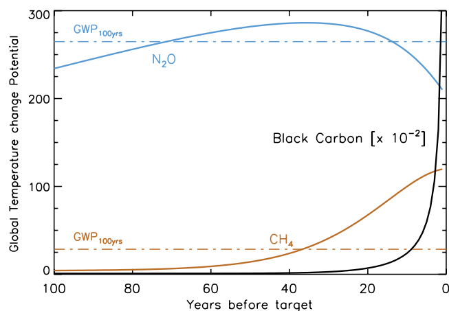
Figure 8.30 | Global Temperature change Potential (GTP( t )) for CH 4 , nitrous oxide and BC for each year from year of emission to the time at which the temperature change target is reached. The (time-invariant) GWP 100 is also shown for N 2 O and CH 4 for comparison.
