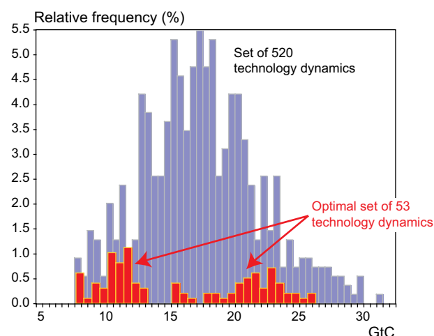
Figure 2.1: Emission impacts of exploring the full spectrum of technological uncertainty in a given scenario without climate policies. Relative frequency (percent) of 130,000 scenarios of full technological uncertainty regrouped into 520 sets of technology dynamics with their corresponding carbon emissions by 2100. Also shown is a subset of 13,000 scenarios grouped into 53 sets of technology dynamics that are all ‘optimal’ in the sense of satisfying a cost minimization criterion in the objective function. See text for further discussion. 1 Gt C = 3.7 Gt CO 2
