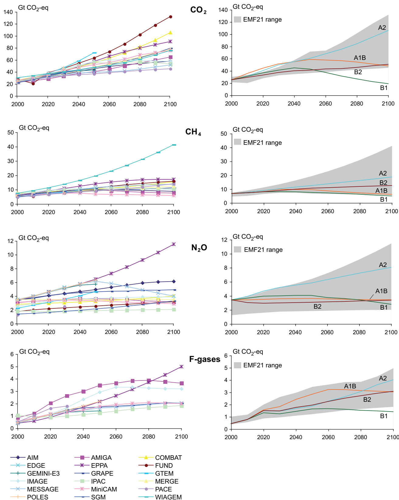
Figure 3.11: Development of baseline emissions in the EMF-21 scenarios (left) and comparison between EMF21 and SRES scenarios (right).
