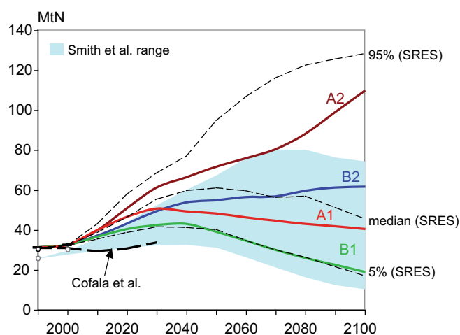
Figure 3.13: \text{NO}_x emission scenarios.
