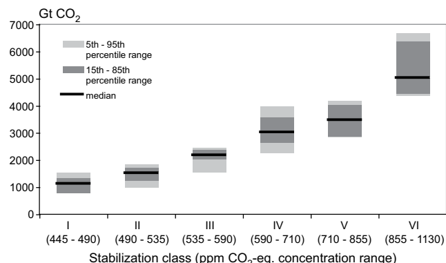
Figure 3.18: Relationship between the scenario's cumulative carbon dioxide emissions (2000–2100) and the stabilization target (stabilization categories I to VI, of Table 3.5).
