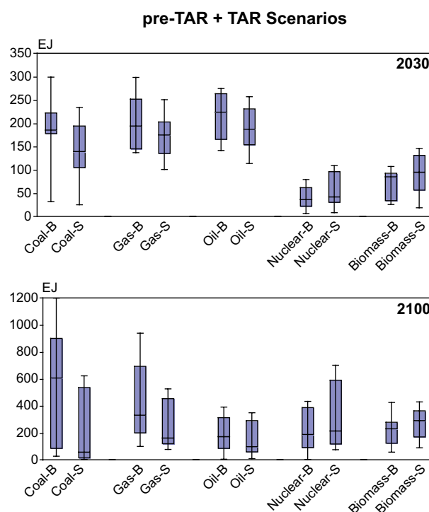
Figure 3.34: Deployment of primary energy technologies across pre-2001 scenarios by 2030 and 2100: Left-side 'error' bars show baseline (non-intervention) scenarios and right-side ones show intervention and stabilization scenarios. The full ranges of the distributions (full vertical line with two extreme tic marks), the 25 th and 75 th percentiles (blue area) and the median (middle tic mark) are also shown.
