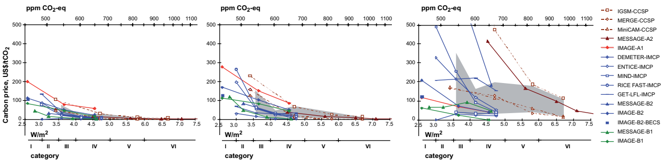
Figure 3.25: Figure 3.25 Relationship between the cost of mitigation and long-term stabilization targets (radiative forcing compared to pre-industrial level, W/m^2 and CO_2 -eq concentrations).
