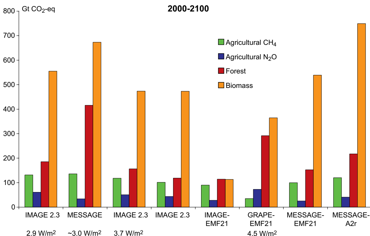
Figure 3.29: Cumulative cost-effective agricultural, forestry, and biomass abatement 2000–2100 from various 2100 stabilization scenarios.
