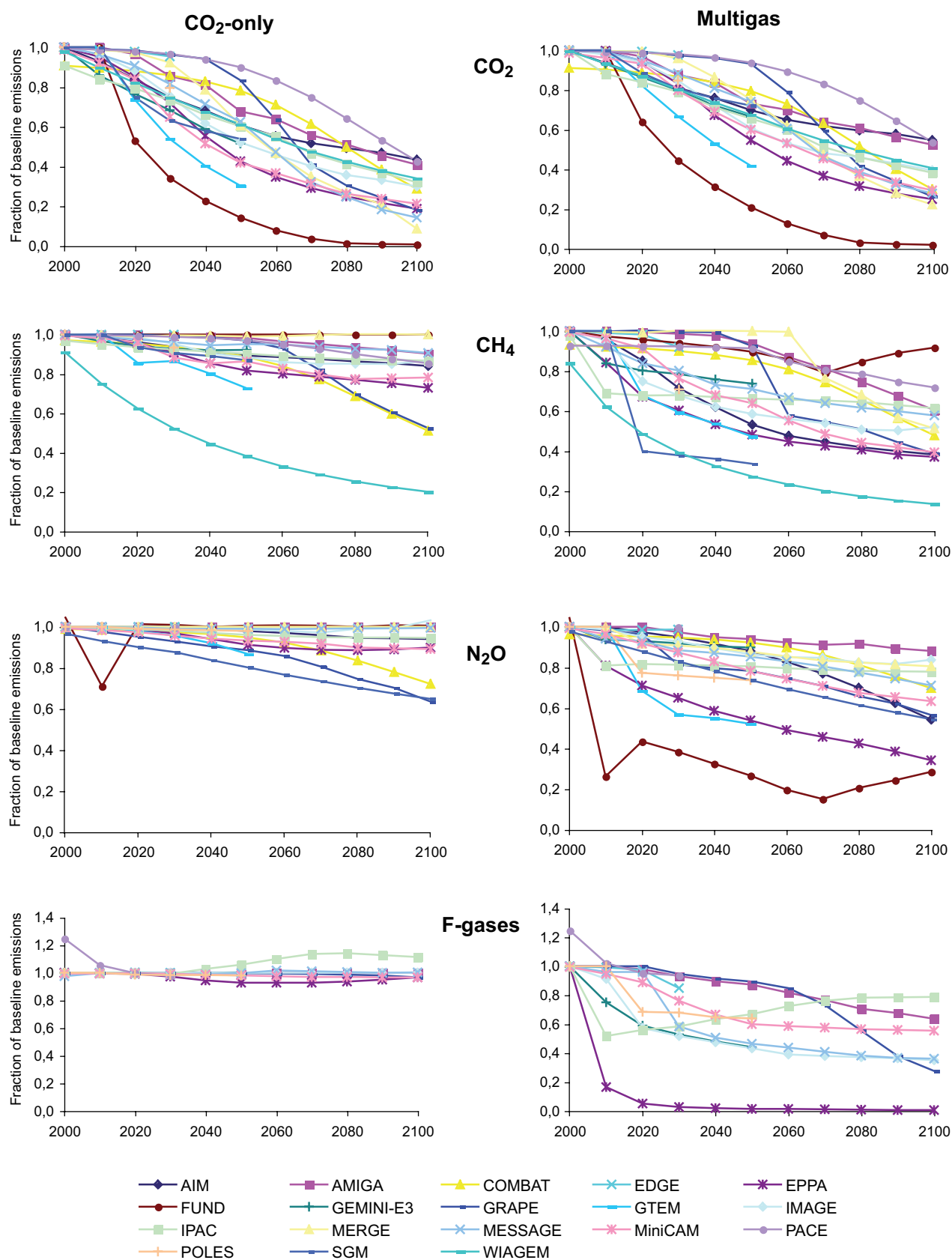
Figure 3.26: Reduction of emissions in the CO 2 -only versus multi-gas strategies.
