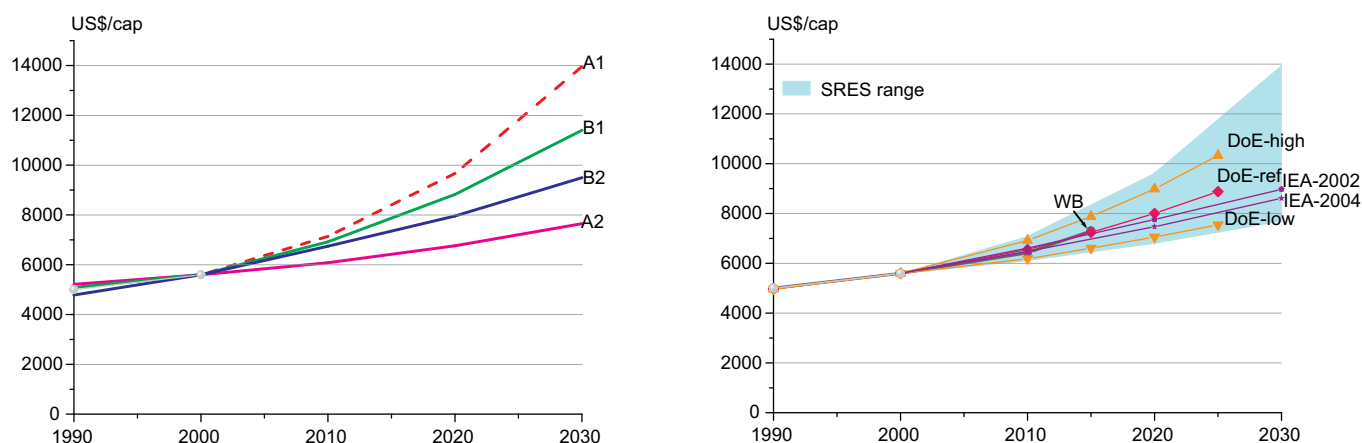
Figure 3.3: Comparison of global GDP growth per person in the SRES scenarios and more recent projections.
