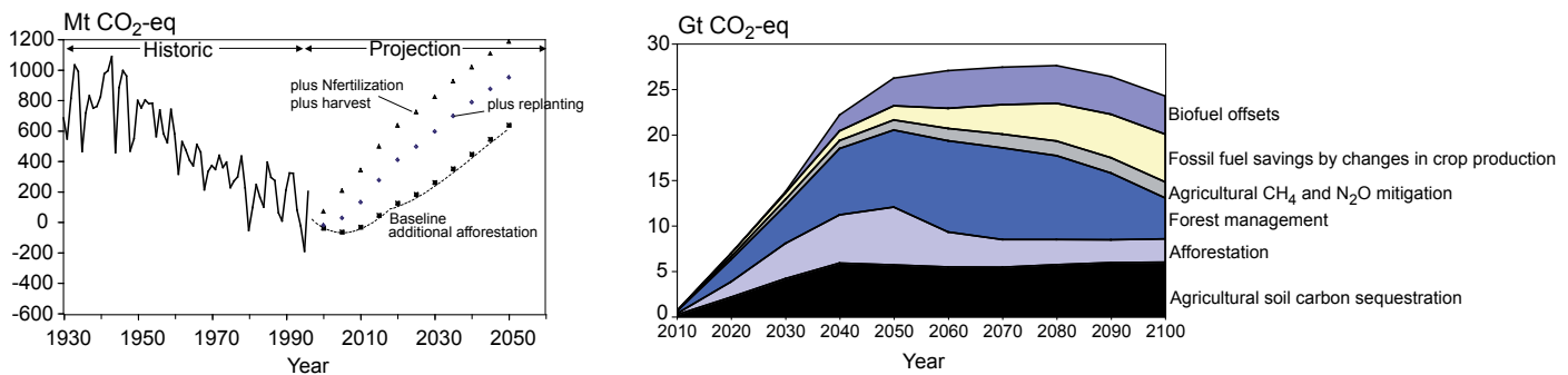
Figure 9.8: OECD North America: technical potential for the forest sector alone for Canada (left, sink is positive) and the economic potential (at 15 US$/tCO 2 e in constant real prices) in the agriculture and forestry sector in the USA (right) Left: Chen et al. , 2000; right: US-EPA, 2005
