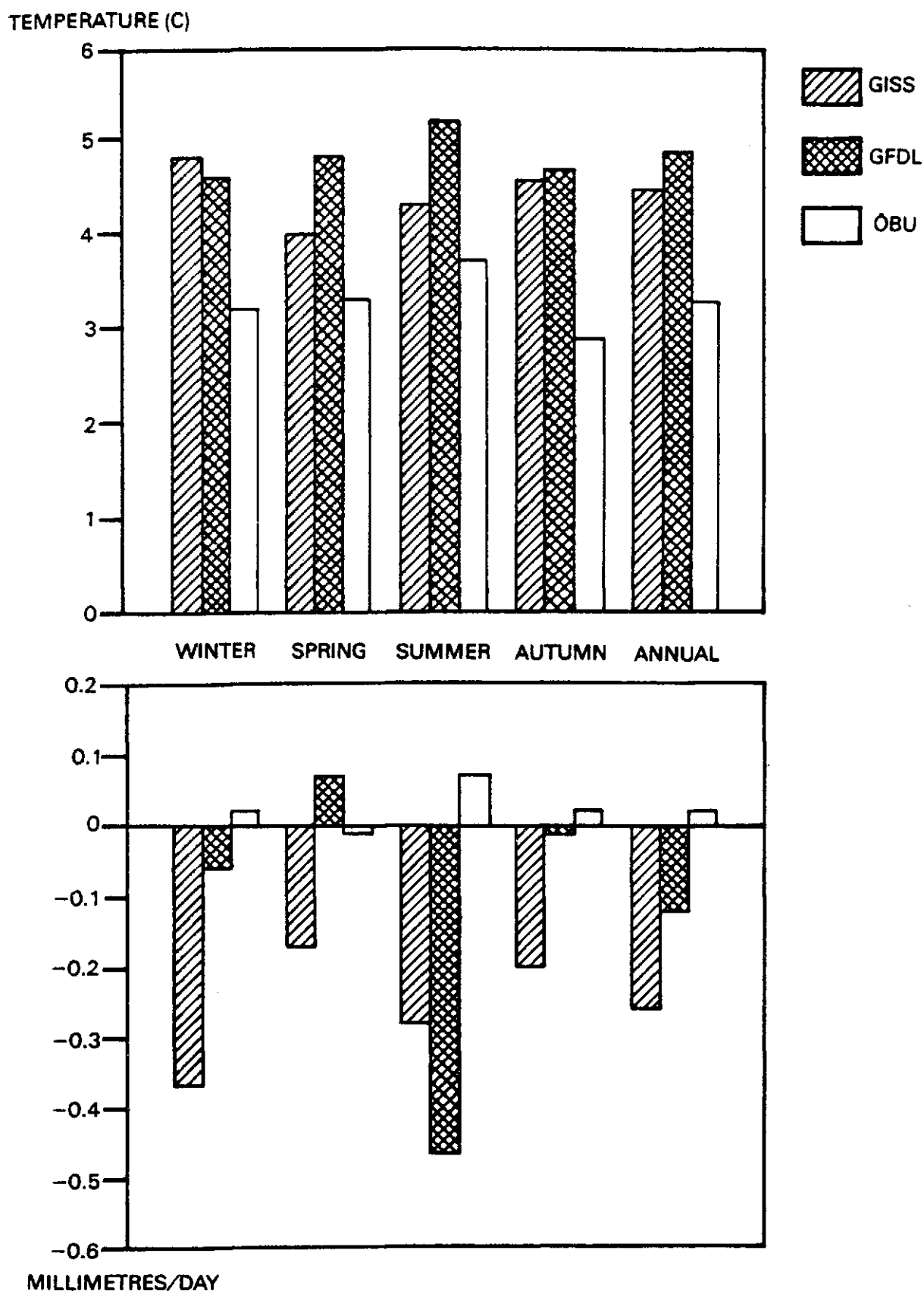
Figure 4.12. GCM-estimated average seasonal and annual changes in temperature (upper) and precipitation (lower) for the grid cells encompassing the Great Plains ( 2 \times \text{CO}_2 minus 1 \times \text{CO}_2 ) (Smith and Tirpak, 1989)
