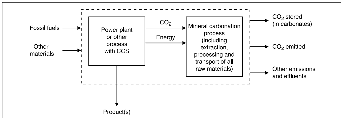
Figure 7.1 Material and energy balances through the system boundaries for a power plant with \text{CO}_2 capture and storage through mineral carbonation. The fossil fuel input provides energy both to the power plant that produces \text{CO}_2 and to the mineralization process (either directly or indirectly via the power plant). The ‘other materials’ input serves all processes within the system boundaries and includes the metal oxide bearing materials for mineralization. The ‘other emissions’ output is made up of the byproducts of the mineralization reaction - silica and possibly water - as well as of non-reacted input materials.
