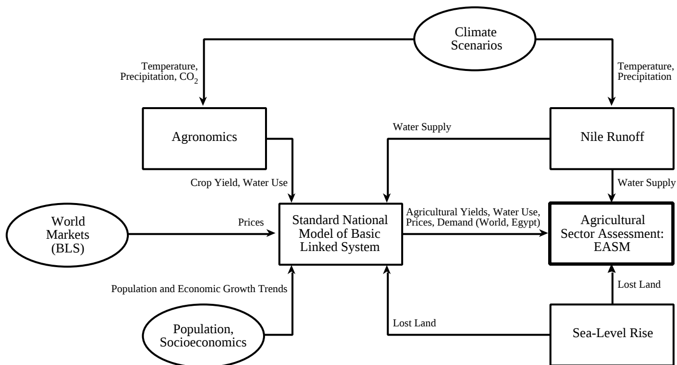
Figure 10-8: Schematic of forward-linkage approach to integrated assessment of climate change impacts on Egypt, using agricultural sector model (Yates and Strzepek, 1998).
