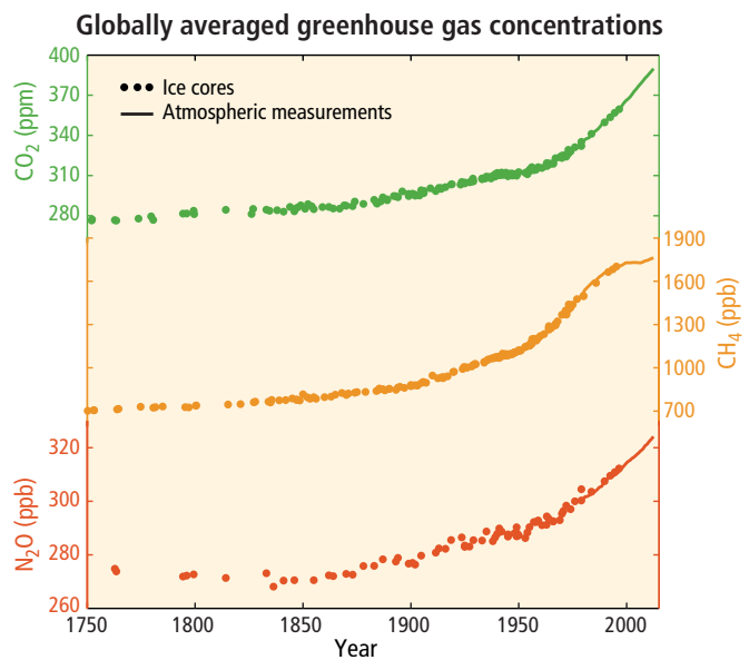
Figure 1.3 | Observed changes in atmospheric greenhouse gas concentrations. Atmospheric concentrations of carbon dioxide (CO 2 , green), methane (CH 4 , orange), and nitrous oxide (N 2 O, red). Data from ice cores (symbols) and direct atmospheric measurements (lines) are overlaid. {WGI 2.2, 6.2, 6.3, Figure 6.11}
