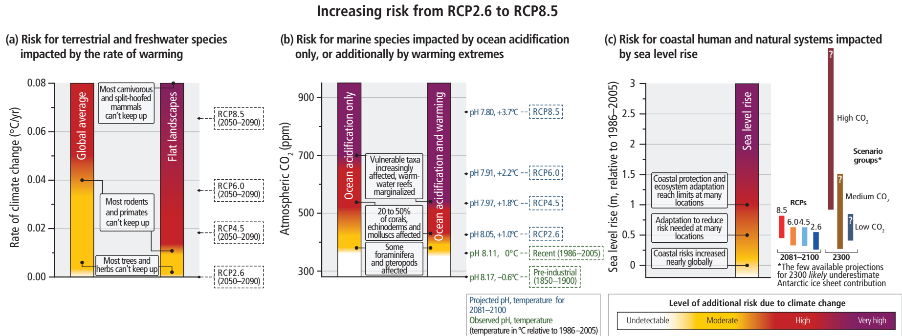
Figure 2.5 | The risks of: (a) disruption of the community composition of terrestrial and freshwater ecosystems due to the rate of warming; (b) marine organisms impacted by ocean acidification (OA) or warming extremes combined with OA; and (c) coastal human and natural systems impacted by sea level rise. The risk level criteria are consistent with those used in Box 2.4 and their calibration is illustrated by the annotations to each panel. (a) At high rates of warming, major groups of terrestrial and freshwater species are unable to move fast enough to stay within the spatially shifting climate envelopes to which they are adapted. The median observed or modelled speeds at which species populations move (km/decade) are compared against the speed at which climate envelopes move across the landscape, given the projected climate change rates for each Representative Concentration Pathway (RCP) over the 2050–2090 period. The results are presented for the average of all landscapes globally, as well as for flat landscapes, where the climate envelope moves especially fast. (b) Sensitivity to ocean acidification is high in marine organisms building a calcium carbonate shell. The risks from OA increase with warming because OA lowers the tolerated levels of heat exposure, as seen in corals and crustaceans. (c) The height of a 50-year flood event has already increased in many coastal locations. A 10- to more than 100-fold increase in the frequency of floods in many places would result from a 0.5 m rise in sea level in the absence of adaptation. Local adaptation capacity (and, in particular, protection) reaches its limits for ecosystems and human systems in many places under a 1 m sea level rise. (2.2.4, Table 2.1, Figure 2.8) [WGI 3.7.5, 3.8, 6.4.4, Figure 13.25, WGII Figure SPM.5, Figure 4-5, Figure 6-10, Box CC-OA, 4.4.2.5, 5.2, 5.3–5.5, 5.4.4, 5.5.6, 6.3]
