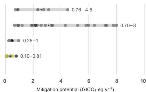
Figure TS.5 | Mitigation potential of response options in 2020–2050, measured in GtCO 2 -eq yr -1 , adapted from Roe et al. (2017).
