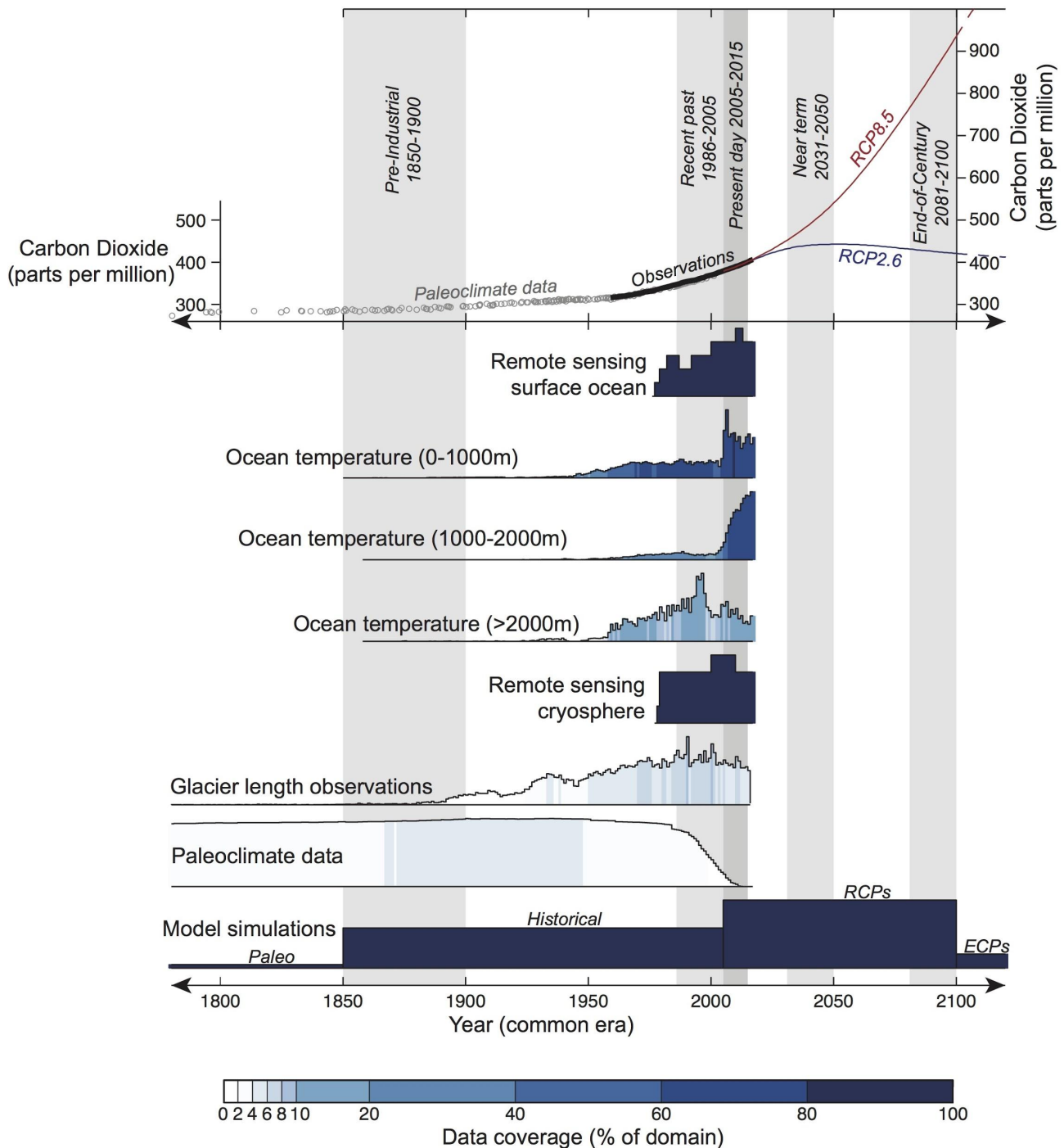
Figure 1.4: Major time periods covered in this Special Report and examples of ocean and cryosphere data coverage over these times. Upper panel displays observed (Keeling et al., 1976) and reconstructed (Bereiter et al., 2015) atmospheric carbon dioxide concentrations, as well as low (RCP2.6) and high (RCP8.5) future projections (Van Vuuren et al., 2011; Section 1.8.2.3). Lower panel gives examples of available data for the ocean and cryosphere (Boyer et al., 2013; Dowell et al., 2013; PAGES2k Consortium, 2017; Section 1.7.2; WGMS, 2017). Heights depict the number of observations, parameters or simulations available through time expressed relative to the maximum data availability, and
